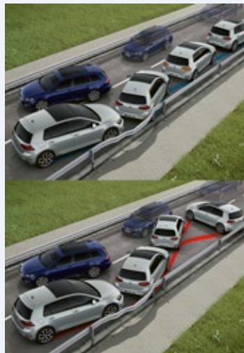
Multikollisionsbroms.
